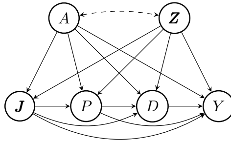
Figure 5: The causal graph for the COMPAS dataset. Z are demographic features, A is race, J juvenile offense counts, P count of prior offenses, D the degree of charge, and Y two year recidivism.
