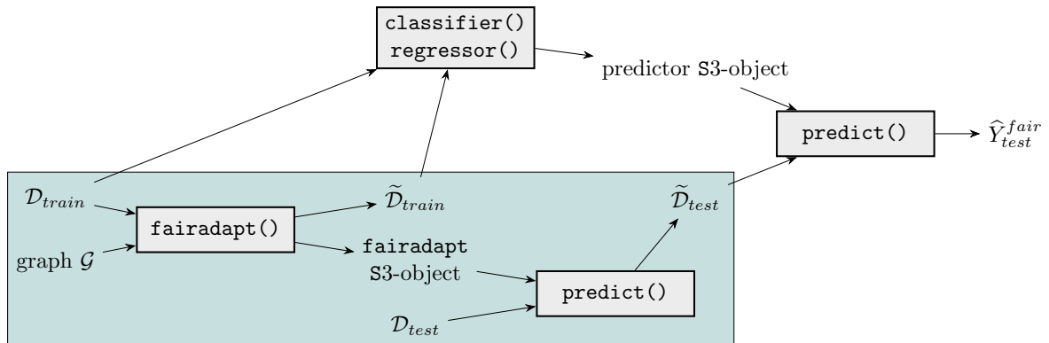
Figure 4: The typical workflow when using fairadapt . The shaded region represents the fair preprocessing which happens within the fairadapt package. Often, this is followed by applying a regressor or a classifier to the transformed data, in order to obtain fair predictions. The latter part is up to the user and not included in fairadapt .
