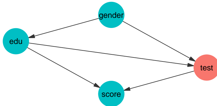
Figure 11: Visualization of the causal graph corresponding to the university admission example introduced in Section 2 with the variable test chosen as a resolving variable and therefore highlighted in red.
