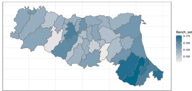
Figure 8: Benchmarked estimates plotted through map() function.
