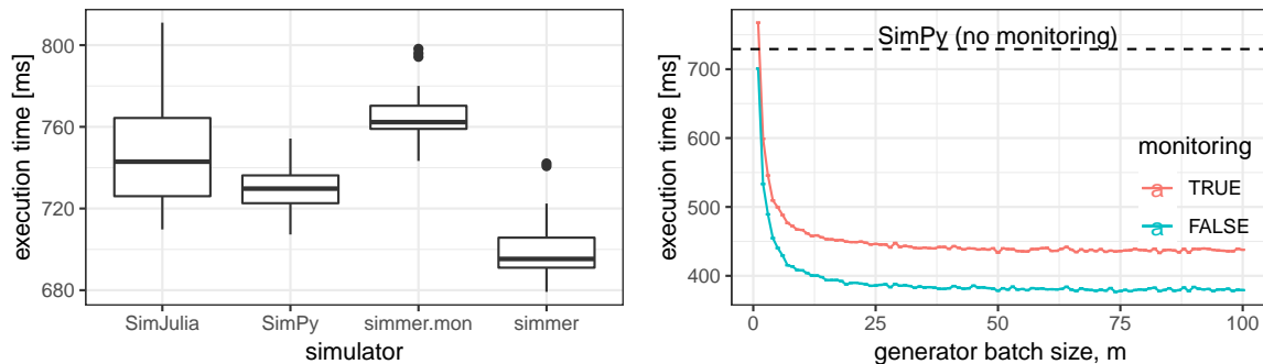
(a) Boxplots for 20 runs of the M/M/1 test with n \leftarrow 1e4 . (b) Performance evolution with the batch size m .
